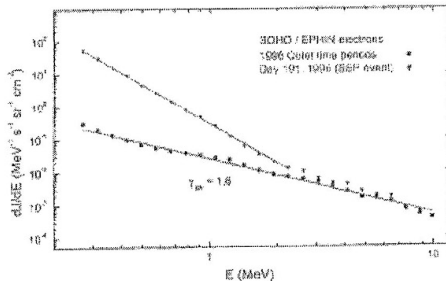
Fig.4. Electron spectrum for 1996 quiet time periods compared with electron spectrum during a SEP event on July 1996.
