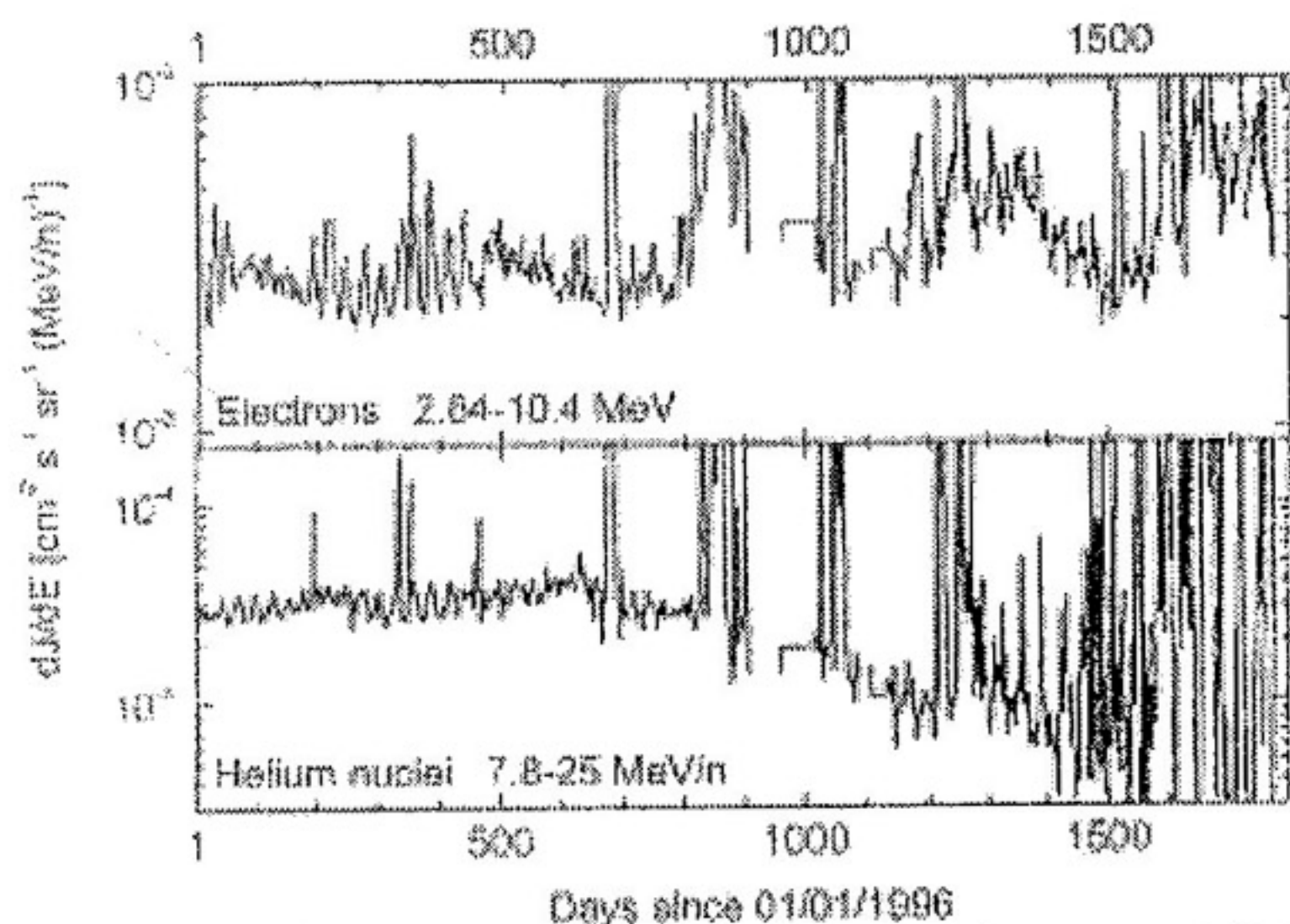
Fig.2. Two-days averaged counting rates of electrons (2.64-10.4 MeV) and Helium (7.8-25 MeV/n) observed by EPHIN.
