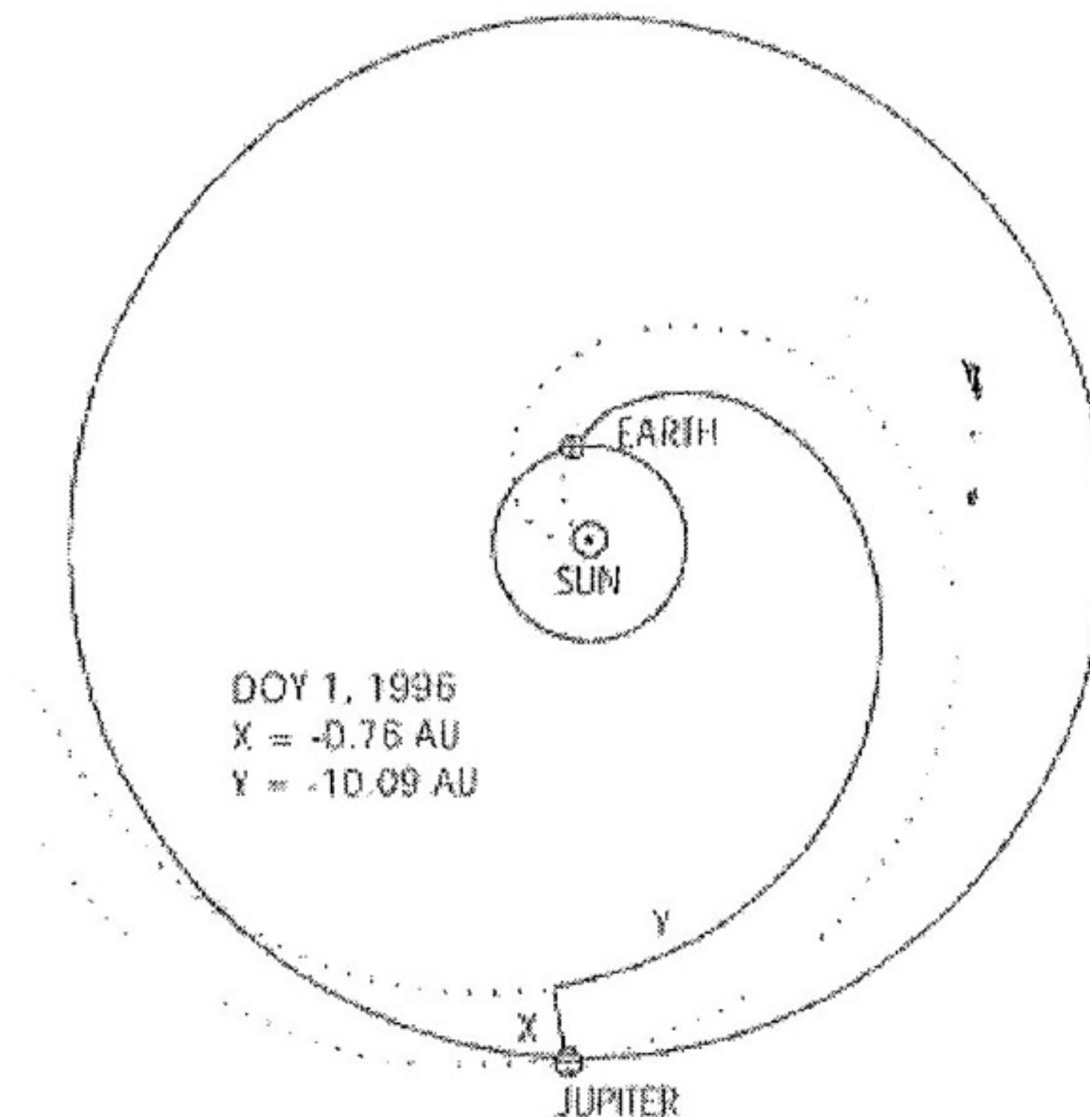
Fig.5. Relative position between Jupiter and Earth in January 1, 1996. IMF lines has been plotted for a solar wind speed of 450 km/s.
