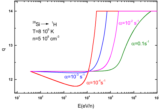
Fig. 2. Evolution of the energy dependence of ^{28}\text{Si} charge states under different acceleration efficiencies, \alpha .
